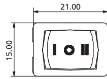
RK5D3Q4_ _ _ _ N ON-OFF-ON
