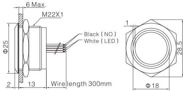
Terminal Type: 24AWG Wire Leading Illumination: Ring Illuminated Blue
