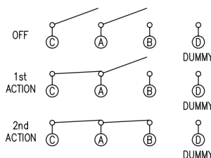
Circuit
